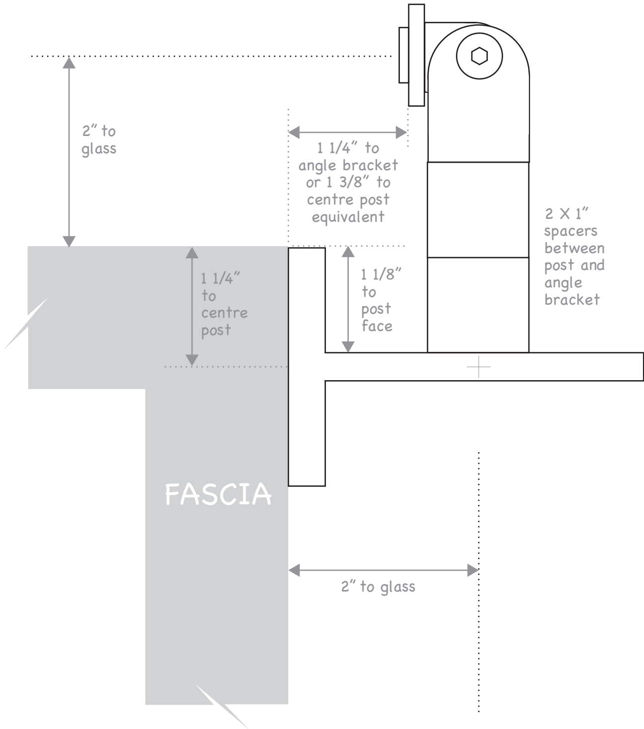
fascia-mount InvisiPost outside 90°
